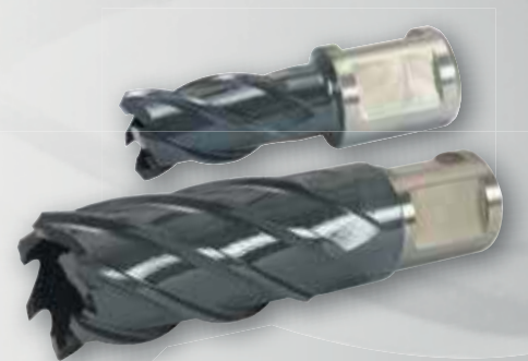
Heavy duty serration with pre- (1) and post-cutter (2)
